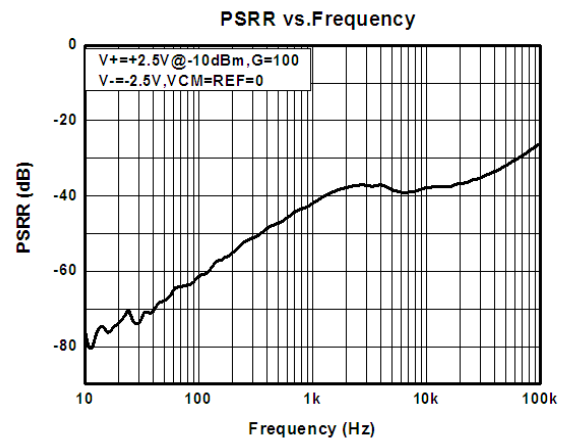
PSRR & Frequency
