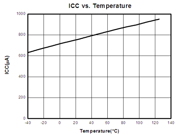
ICC & Temperature
