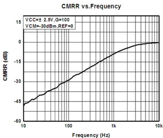
CMRR & Frequency
