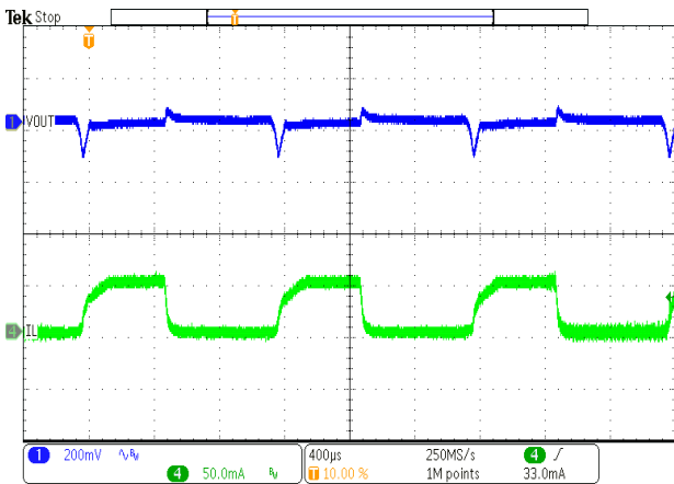
Figure 7. Load transient
