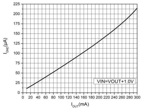
Figure 4. I GND vs I OUT
