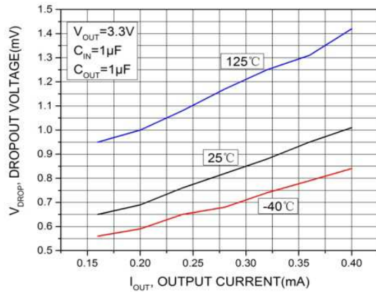
Figure 6. Dropout Voltage vs Output Current V OUT =3.3V
