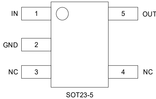
Figure 2. Top View
