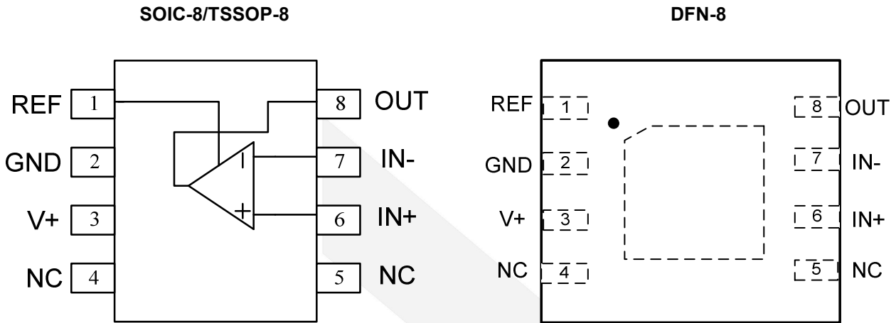
Figure 1 Pin Assignment
