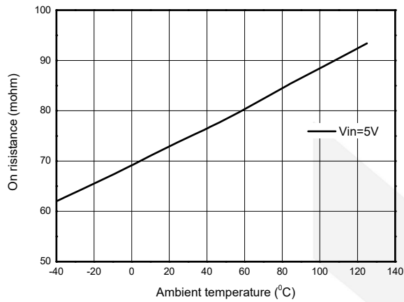
On Resistance vs. Ambient Temperature
