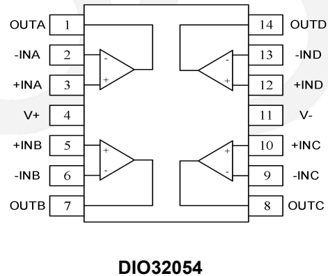
Figure 1. Pin Assignment
