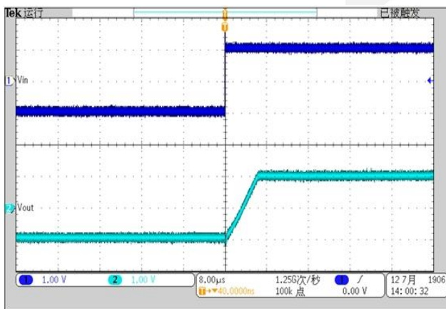
Slew Rate
