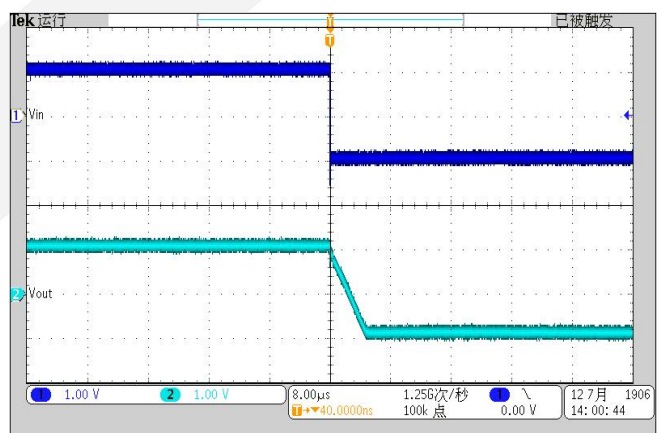
Slew Rate
