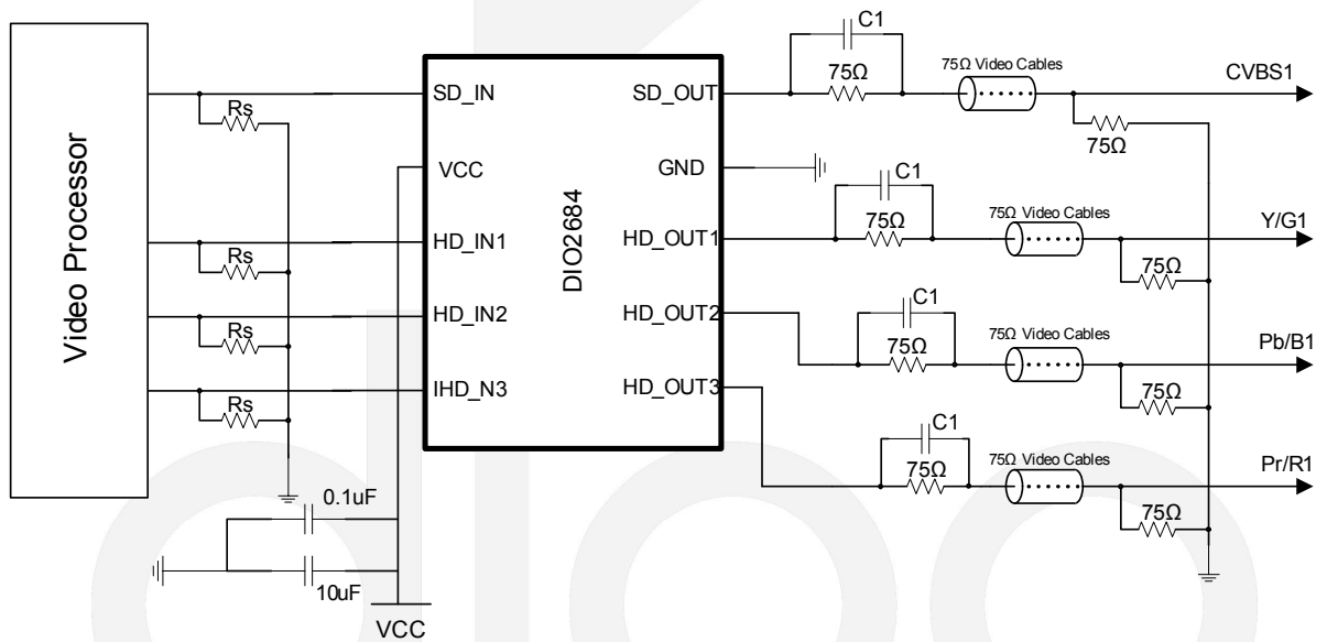
Figure 3 Input and Output DC-Coupling Application
