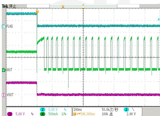
Full-Load to Short-Circuit Transient Response for DIO7004HC (Iload=0.7A, Vin=5V)
