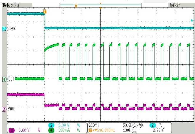
No-Load to Over-Load Transient Response for DIO7004HC (Vin=5V, R=1ohm)
