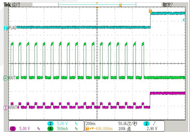
Over-Load to No-Load Recovery Response for DIO7004HC (Vin=5V, R=1ohm)
