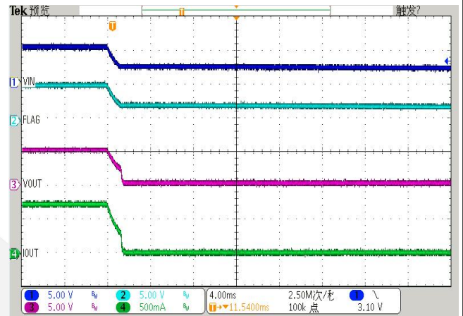
UVLO Turn Off for DIO7004HC (Iload=0.7A, Vin=5V, R=7ohm)
