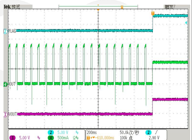
Short-Circuit to Full-Load Recovery Response for DIO7004HC (Iload=0.7A, Vin=5V)
