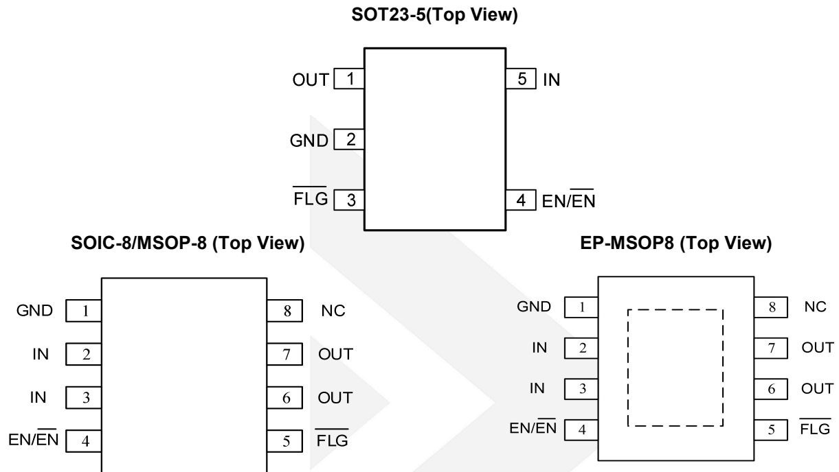
Figure 1 Pin Assignment
