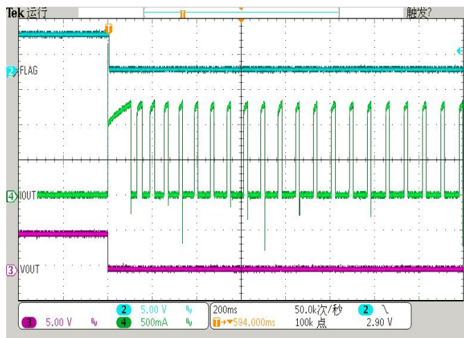
No-Load to Short-Circuit Transient Response for DIO7004HC (Vin=5V)
