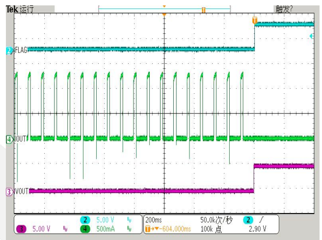
Short-Circuit to No-Load Recovery Response for DIO7004HC (Vin=5V)
