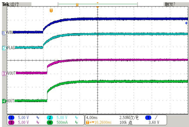
UVLO Turn On for DIO7004HC (Iload=0.7A, Vin=5V, R=7ohm)
