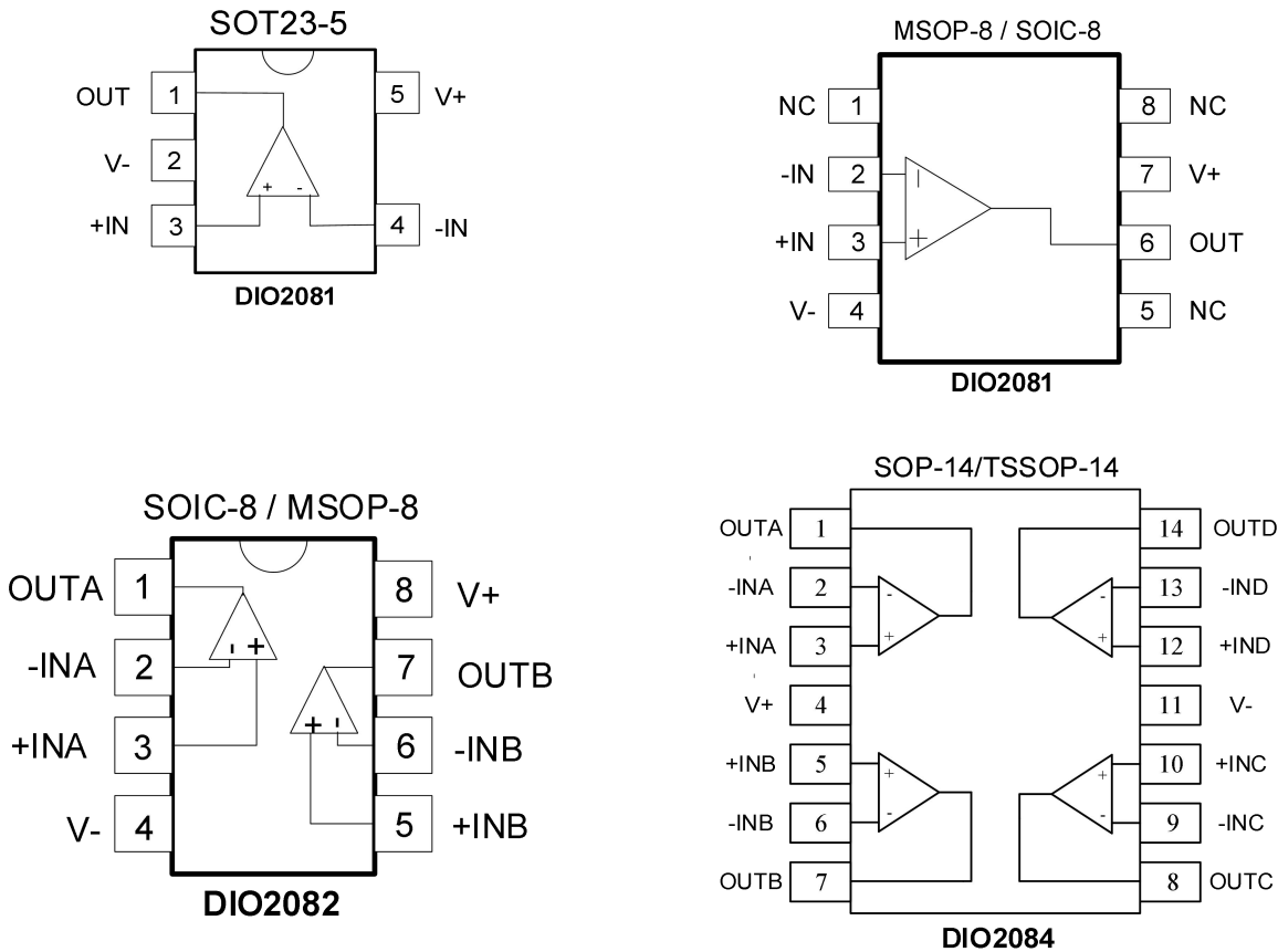
Figure 1 Top View
