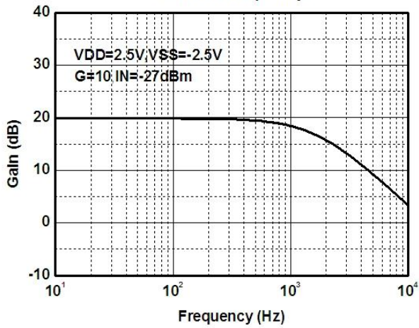
GBW vs.Frequency
