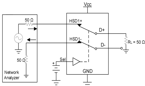
Figure 14. Channel-to-channel crosstalk
