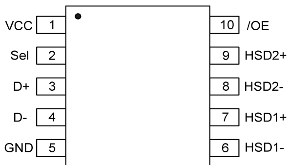
Figure 1. MSOP-10 (Top view)
