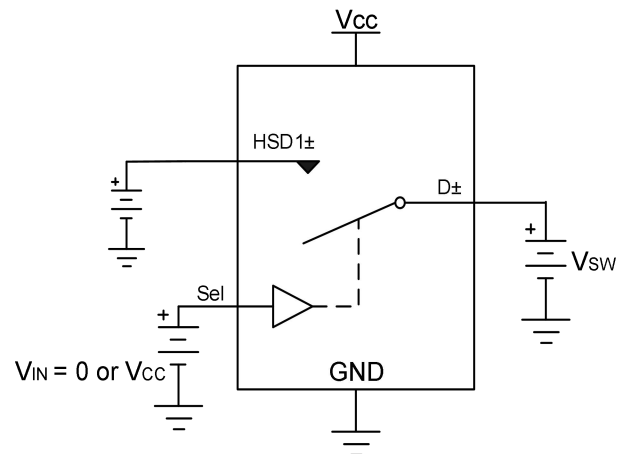
Figure 11. Switch off leakage
