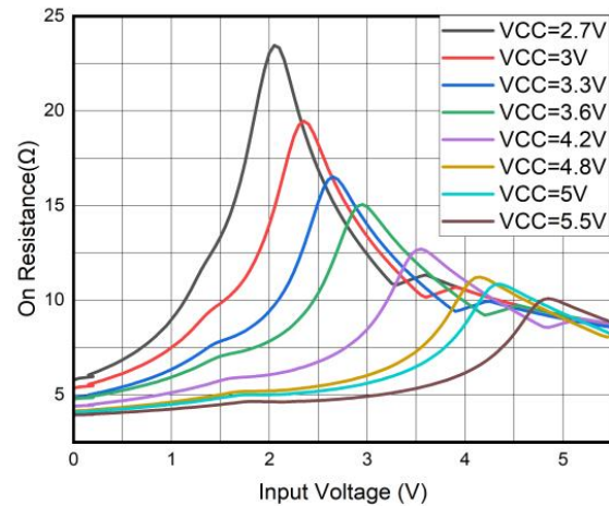
Figure 7. On resistance vs. Input voltage
