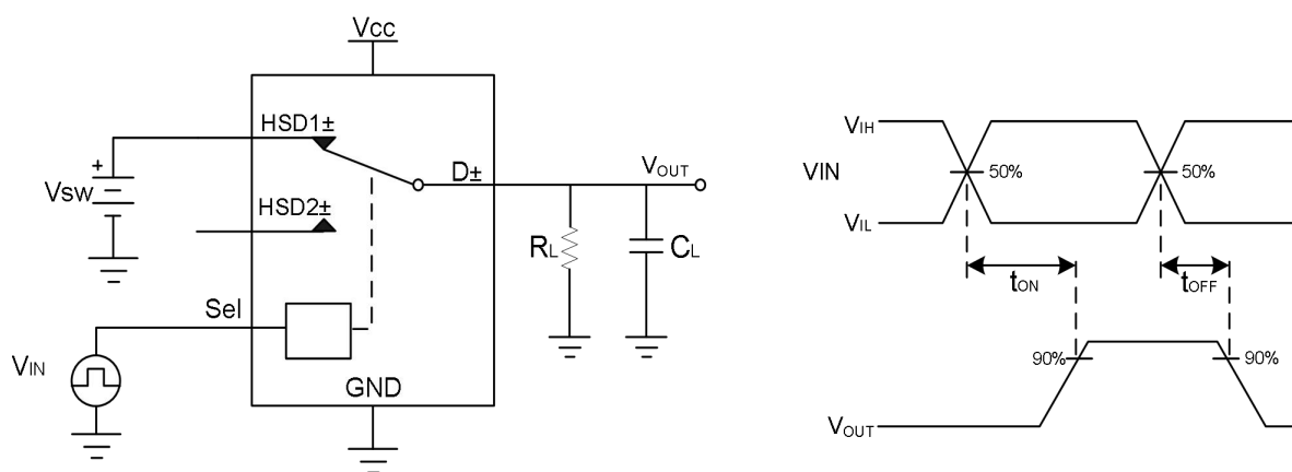
Figure 17. Turn-on/Turn-off
