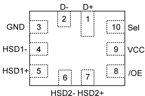
Figure 3. QFN1.4x1.2-10 (Top view)
