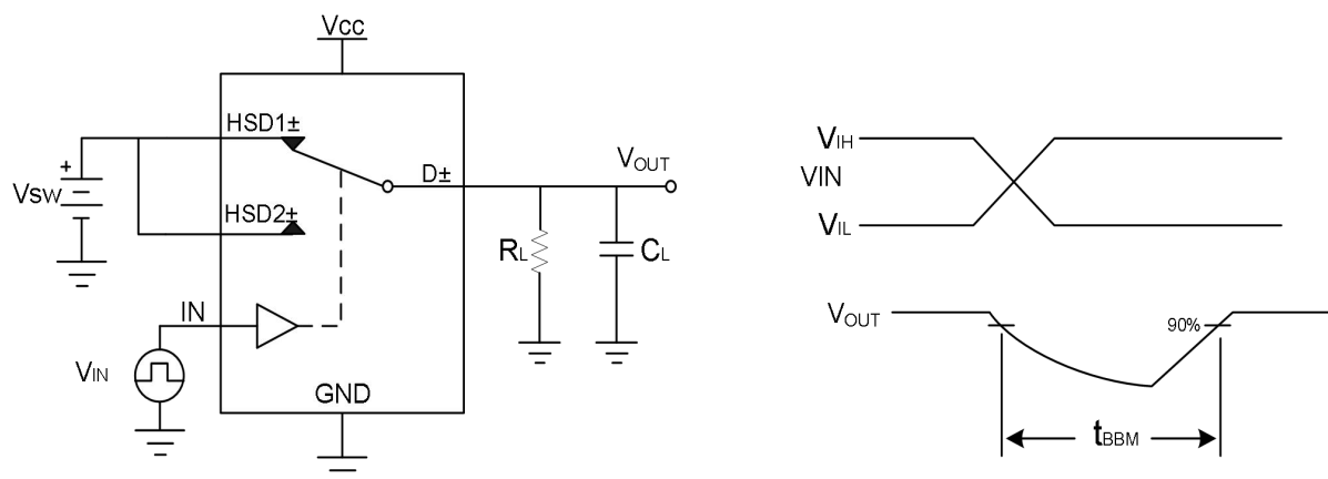
Figure 16. Break-before-make
