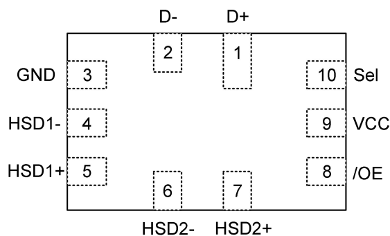
Figure 2. QFN1.4x1.8-10 (Top view)
