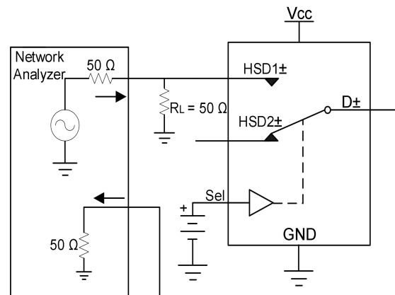
Figure 15. Off-isolation
