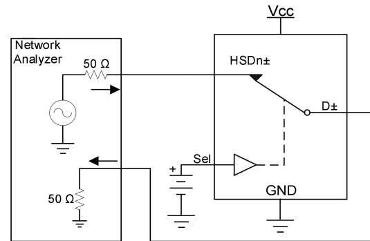
Figure 13. Bandwidth
