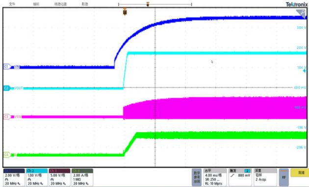
Figure 6. VIN start
