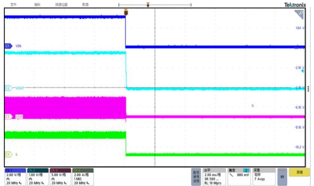
Figure 9. VEN drop
