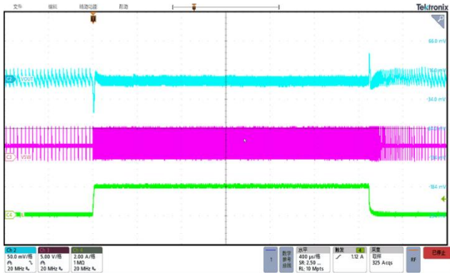
Figure 10. Load transient
