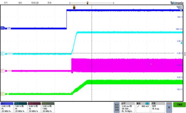
Figure 8. VEN start
