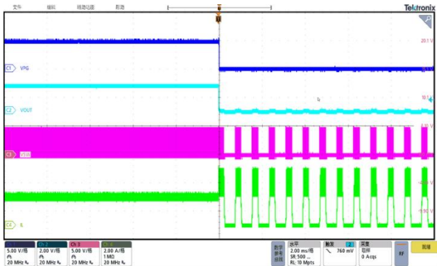
Figure 14. Short circuit protection
