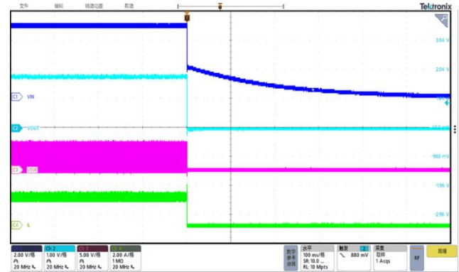
Figure 7. VIN drop
