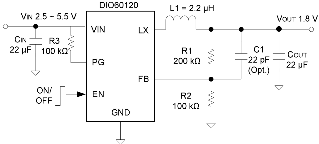
Figure 17. Typical application
