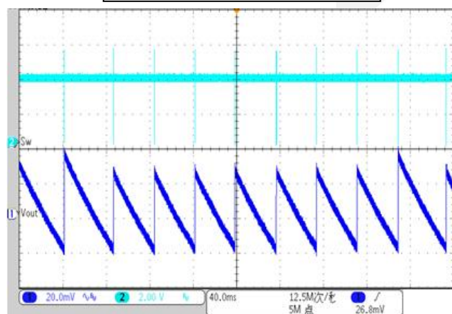
Output Ripple V_{\text{IN}}=3.6\text{V} V_{\text{OUT}}=5\text{V} No Load
