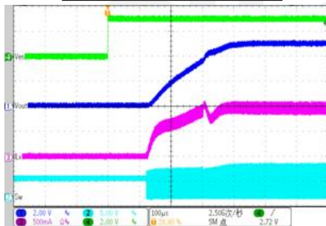
Startup through Enable V_{\text{IN}}=3.6\text{V} V_{\text{OUT}}=5\text{V} R_{\text{LOAD}}=8.2\Omega
