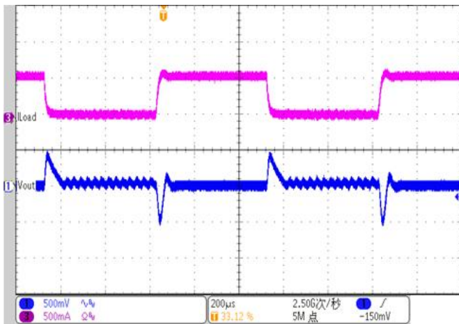
Load Transient Vin=3.6V Vout=5V Load=0A->0.6A
