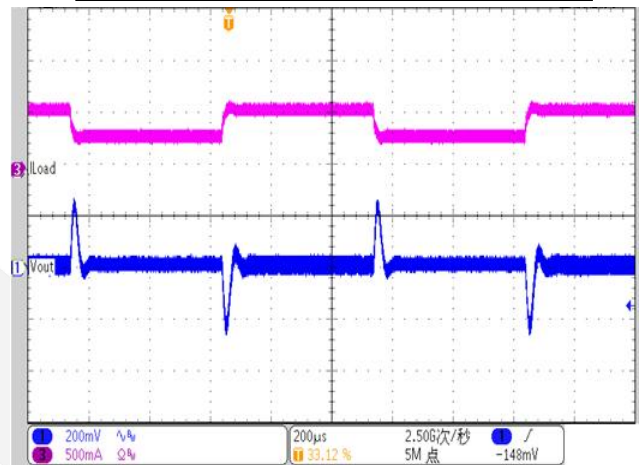
Load Transient Vin=3.6V Vout=5V Load=0.3A->0.6A
