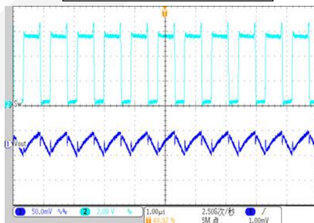
Output Ripple V_{\text{IN}}=3.6\text{V} V_{\text{OUT}}=5\text{V} Load=0.6A
