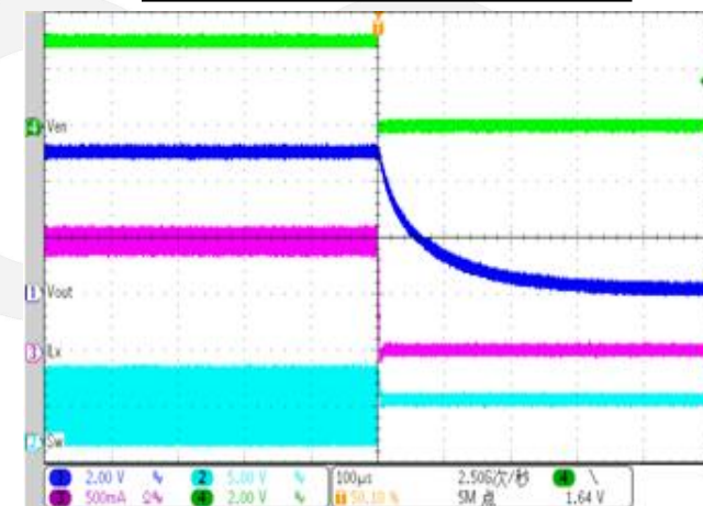
Shutdown through Enable V_{\text{IN}}=3.6\text{V} V_{\text{OUT}}=5\text{V} R_{\text{LOAD}}=8.2\Omega
