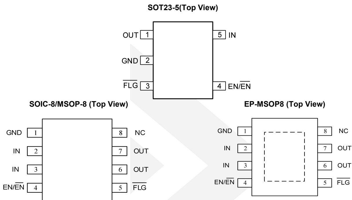
Figure 1 Pin Assignment
