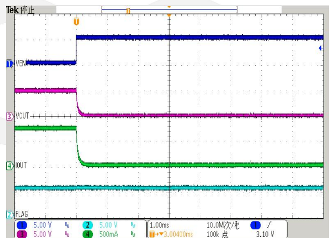
EN Turn Off ( I_{load}=0.7\text{A} , V_{in}=5\text{V} , R=7\text{ohm} )
