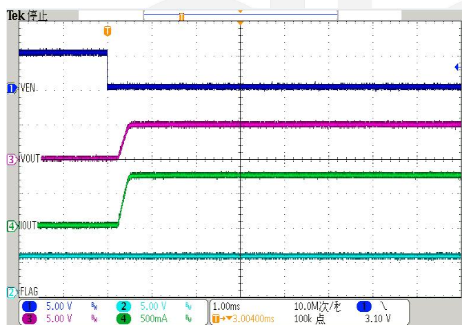
EN Turn On ( I_{load}=0.7\text{A} , V_{in}=5\text{V} , R=7\text{ohm} )
