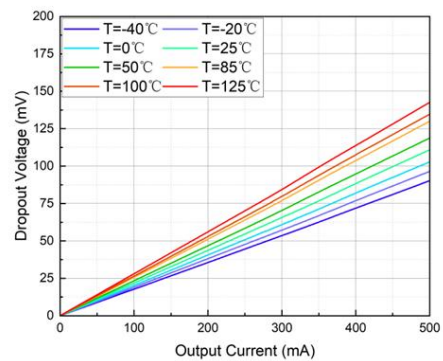
Figure 2. Dropout voltage vs. I_{OUT} at V_{OUT} = 5.5\text{ V}
