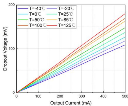
Figure 1. Dropout voltage vs. I_{OUT} at V_{OUT} = 3.3\text{ V}
