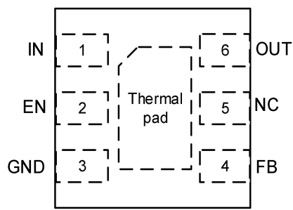
Adjustable DFN2*2-6 (Top view) DIA7855BGADJCD6
