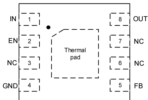
Adjustable DFN3*3-8 (Top view) DIA7855BADJCD8
