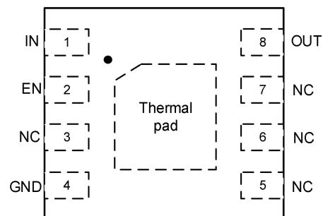
Fixed DFN3*3-8 (Top view) DIA7855BaaCD8
