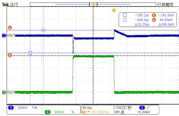
Figure 26. Load transient response at load step from 1 mA to 300 mA, V_{OUT} = 3.3 \text{ V}
