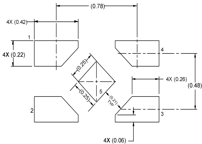
RECOMMENDED LAND PATTERN (Unit: mm)
