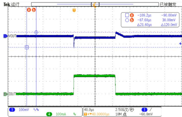
Figure 27. Load transient response at load step from 1 mA to 150 mA, V_{OUT} = 3.3 \text{ V}
