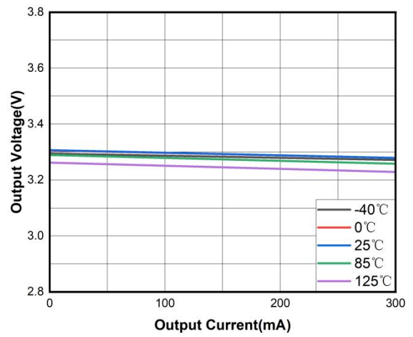
Figure 23. Load regulation vs. Output current
