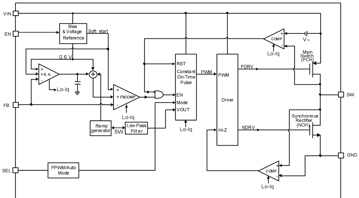
Figure 18. Block diagram
