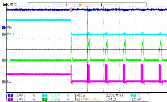
Figure 17. Short-circuit protection
