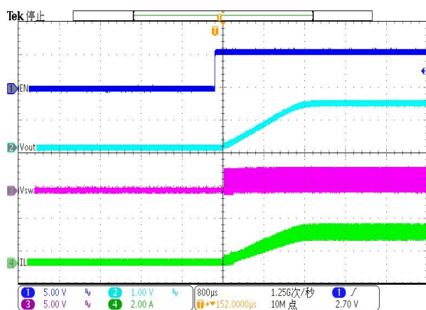
Figure 11. Enable start-up
