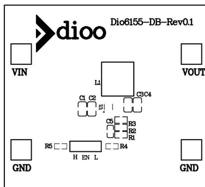
Figure 22. Top Assembly
