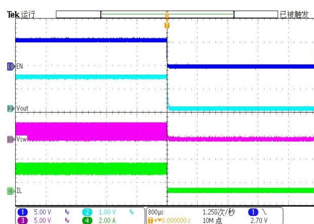
Figure 12. Enable shut-down
