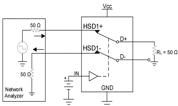
Figure 14. Channel-to-channel crosstalk
