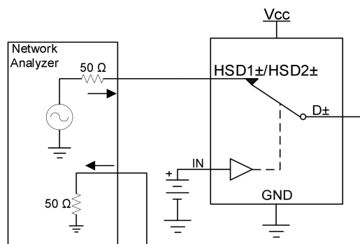
Figure 13. Bandwidth
