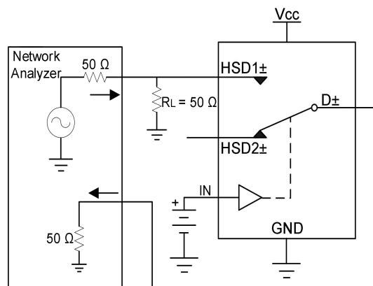
Figure 15. Off-isolation
