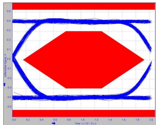
Figure 5. 480 Mbps with USB switch in signal path
