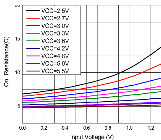
Figure 8. On-resistance vs. Input voltage
