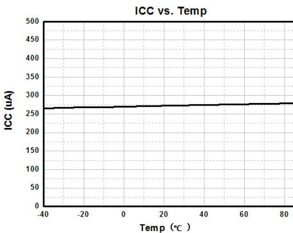
Figure 8. I_{CC} vs. Temp
