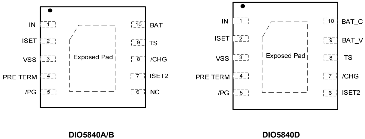
Figure 1. DFN2*2-10 (Top view)
