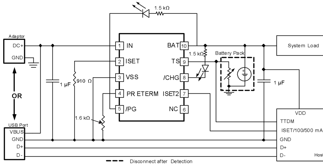
Figure 3. Typical applications for DIO5840A/B
