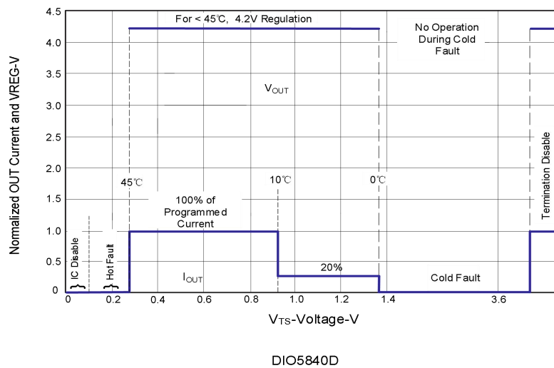
Figure 2. Operation over TS bias voltage
