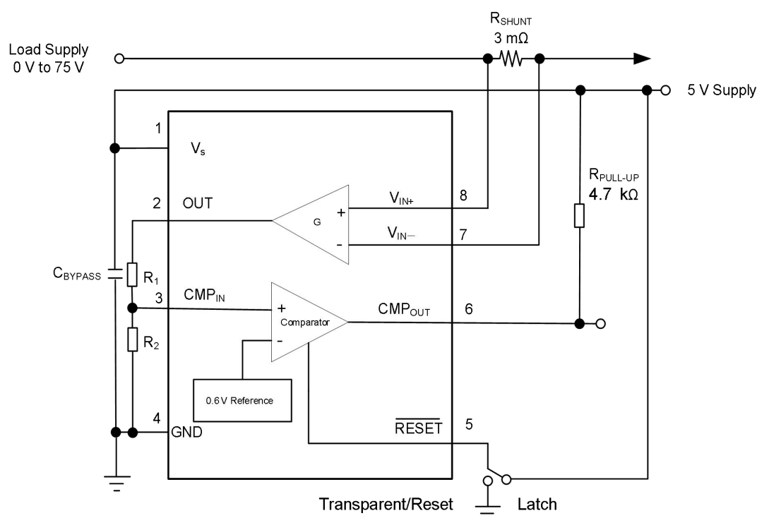
Figure 8. DIO221X basic connections
