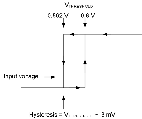
Figure 6. Comparator hysteresis
