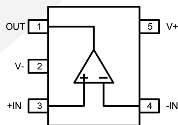
DIO29001 SOT23-5/SC70-5
