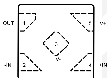
DIO29001 DFN0.8*0.8-4
