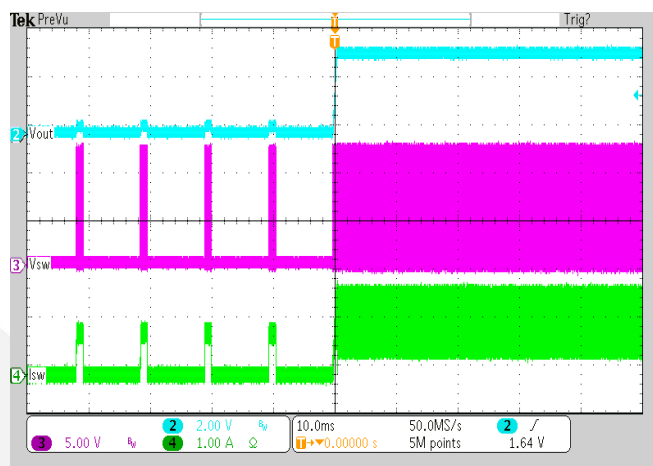
Figure 9 Short Circuit Recovery (Vin=12V, Vout=3.3V, Load=1A)
