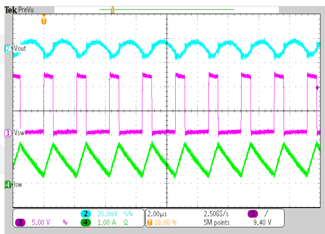
Figure 7 Ripple (Vin=12V, Vout=3.3V, Load=1A)
