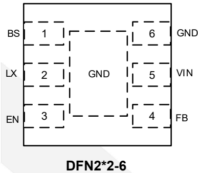
Figure 1 Pin Assignment (Top View)
