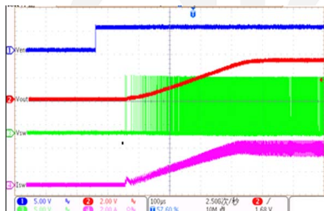
Start up from Enable ( V_{IN}=12V, V_{OUT}=3.3V, Load=1\Omega )
