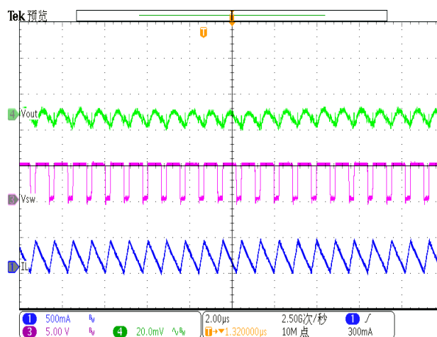
Figure 3. Switching Waveform at Heavy Load
