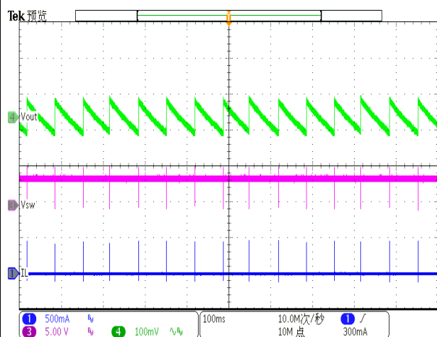
Figure 2. Switching Waveform at Light Load
