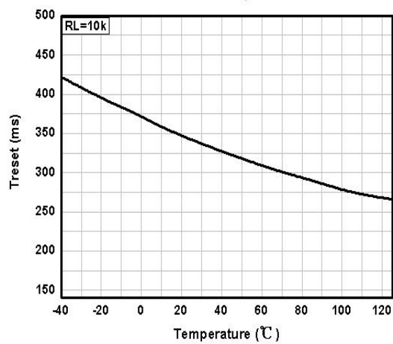
Treset vs. Temperature
