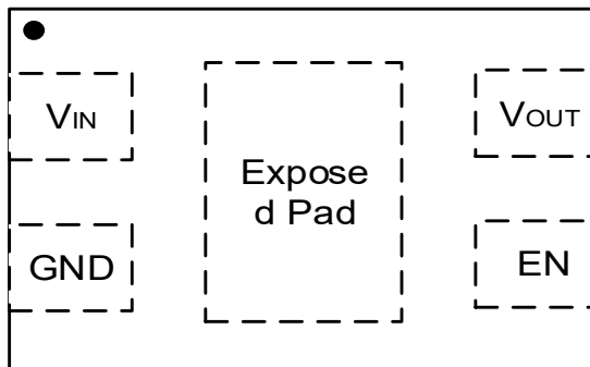
Figure 1 Pin Assignment
