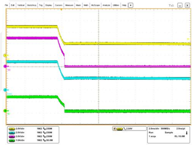
Figure 17. UVLO
