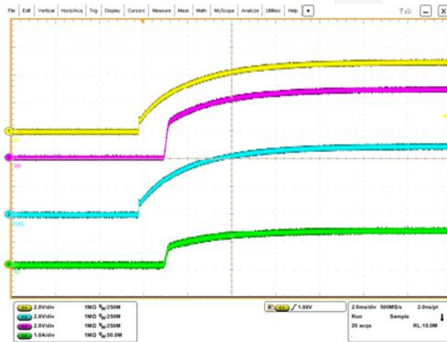
Figure 16. UVLO
