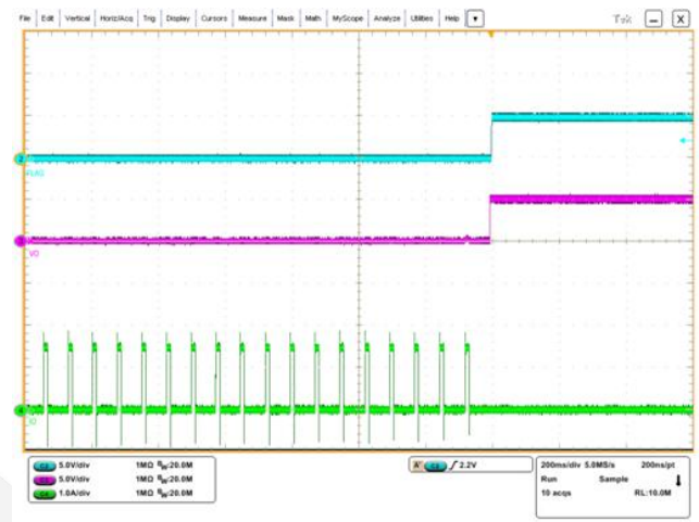
Figure 15. Short recovery
