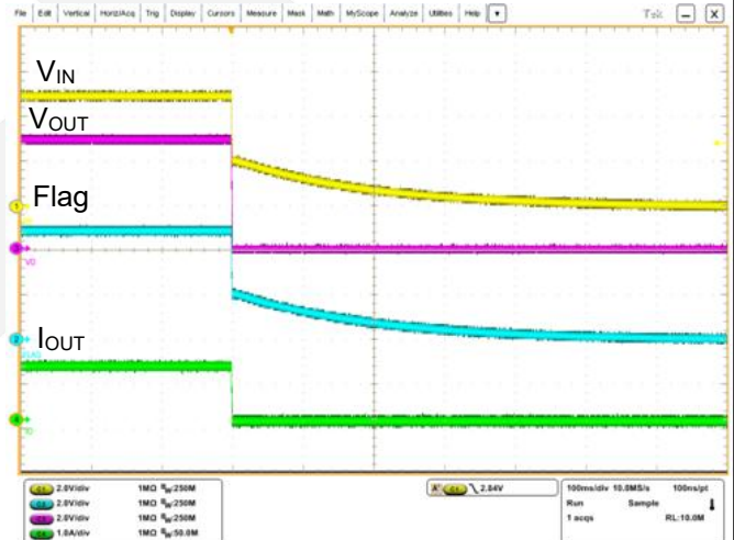
Figure 11. VIN Shut-down
