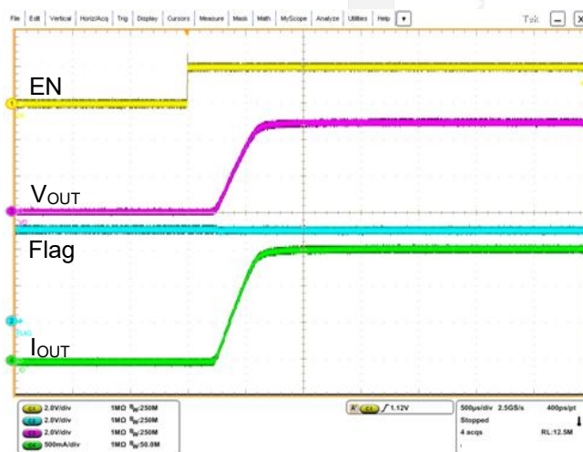
Figure 12. EN Start-up
