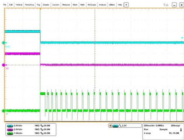
Figure 14. Short protection
