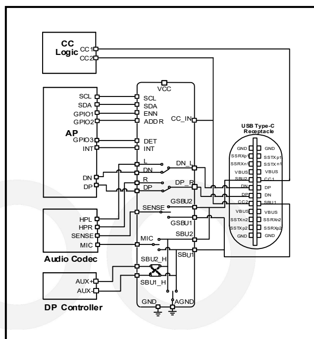
Figure 1. Application Block Diagram
