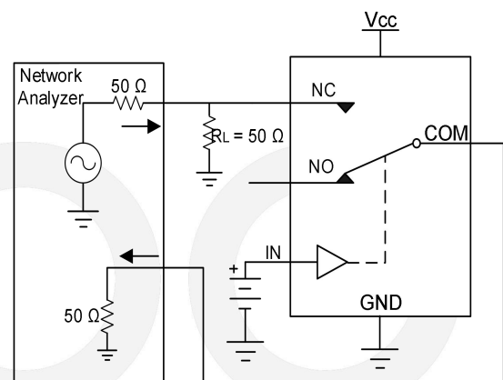
Figure 15. Off-isolation
