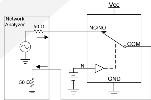
Figure 13. Bandwidth
