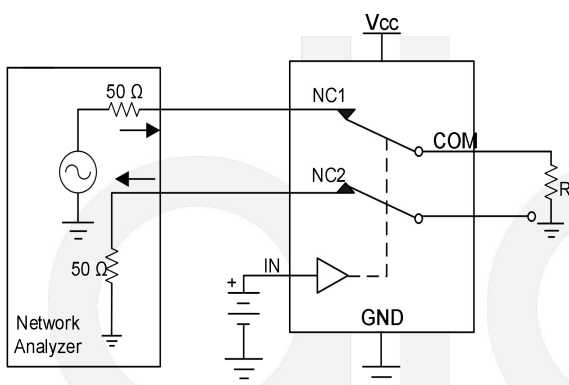
Figure 14. Channel-to-channel crosstalk
