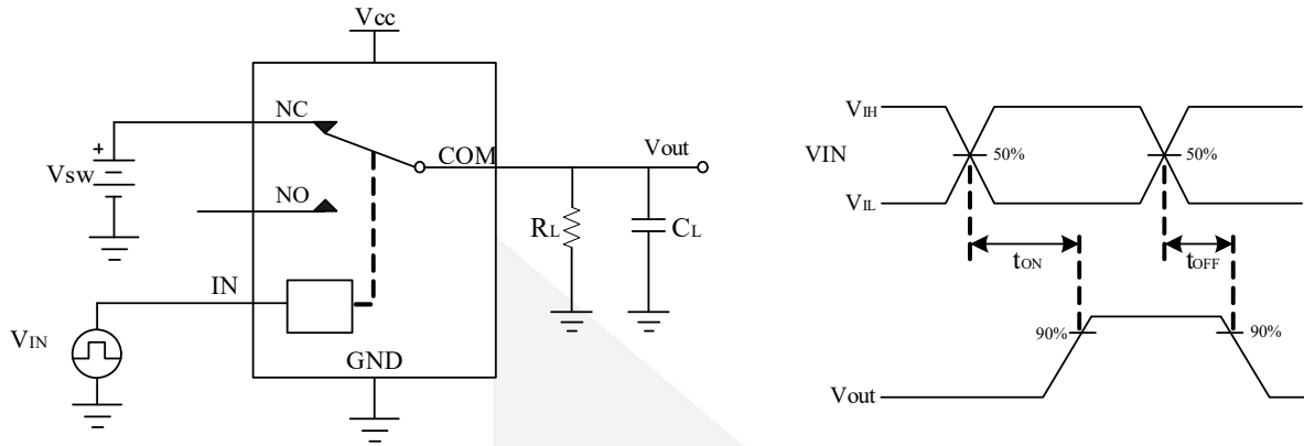
Figure 9 Turn-On/Turn-Off
