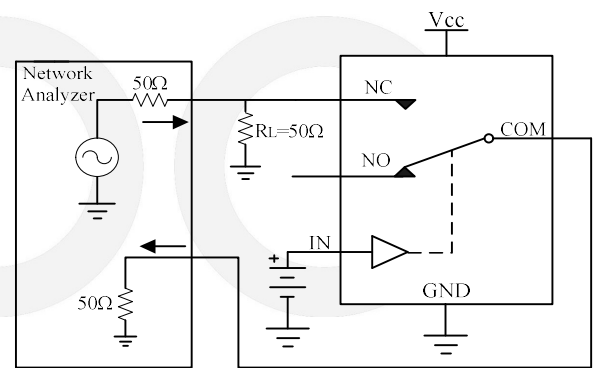
Figure 7 Off-isolation
