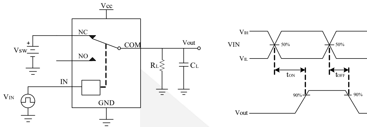
Figure 9 Turn-On/Turn-Off
