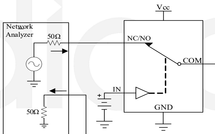
Figure 5 Bandwidth
