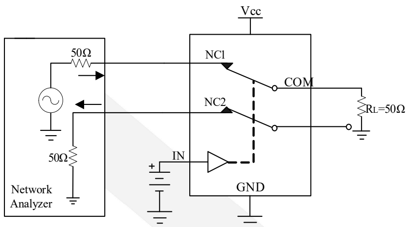
Figure 6 Channel-to-channel crosstalk
