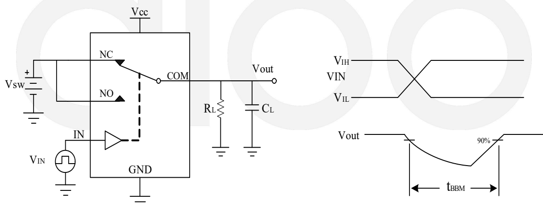
Figure 8 Break-Before-Make
