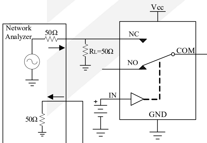
Figure 7 Off-isolation
