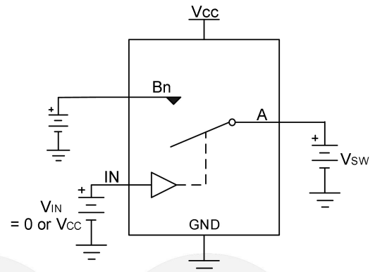
Figure 4. Switch-off leakage
