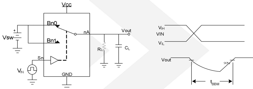
Figure 9. Break-before-make
