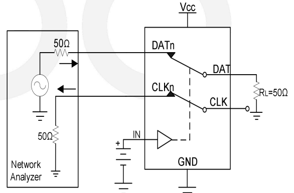
Figure 6. Channel-to-channel crosstalk
