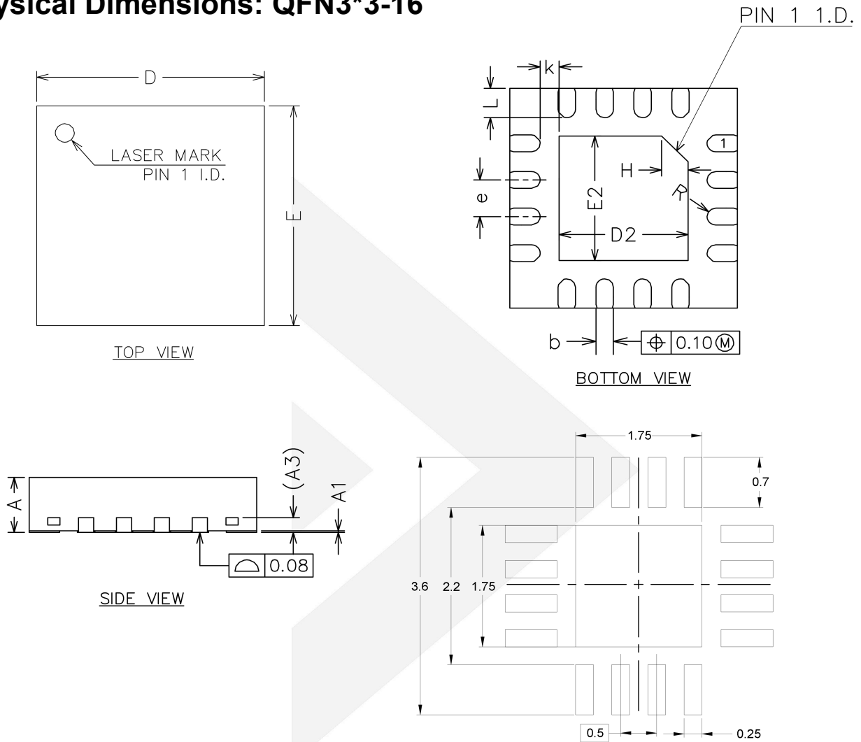
RECOMMENDED LAND PATTERN(Unit:mm)
