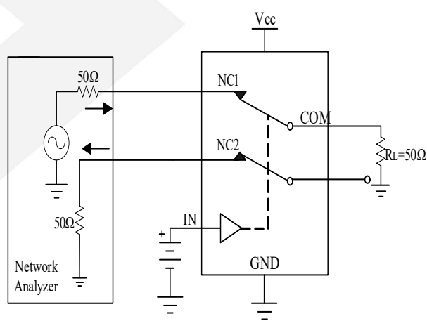
Figure 6 Channel-to-channel crosstalk
