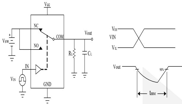
Figure 8 Break-Before-Make
