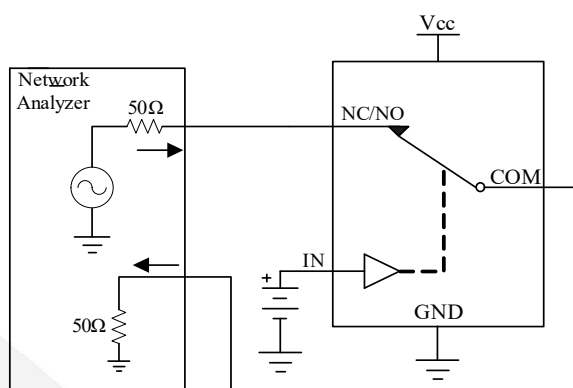
Figure 5 Bandwidth
