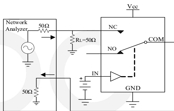
Figure 7 Off-isolation
