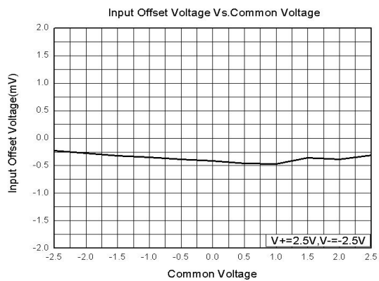
Figure 12 Input offset voltage vs. Common voltage
