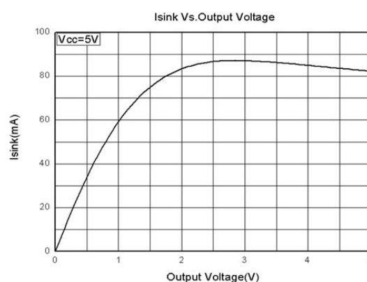
Figure 8 I_{SINK} vs. Output voltage
