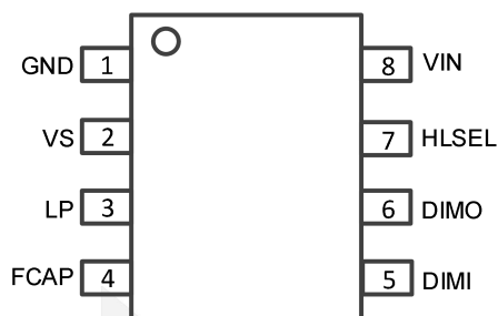
SOIC-8 Top view
