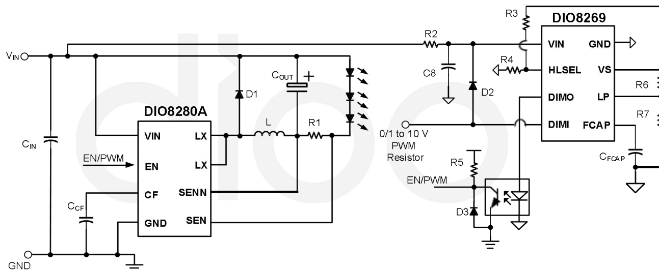
Figure 3. High clamp mode application
