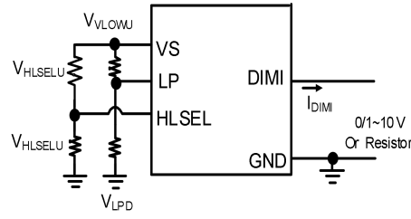
Figure 14. DIMI current setting
