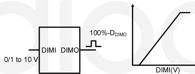
Figure 7. 0/1~10 V dimming
