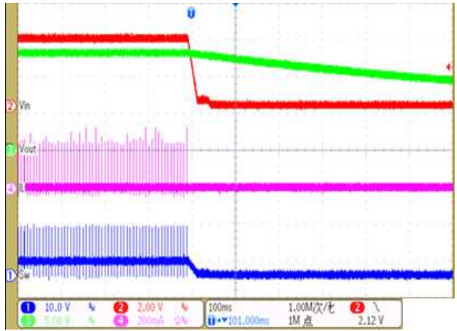
Figure 7. Power Off @ No Load
