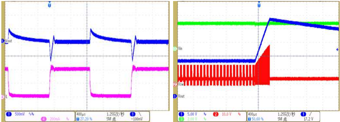
Figure 12. Load Transient (Load=0->400mA) Figure 13. Output Over Voltage Protection Load=0.01A
