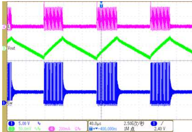
Figure 10. Ripple Burst mode @ Load=0.03A
