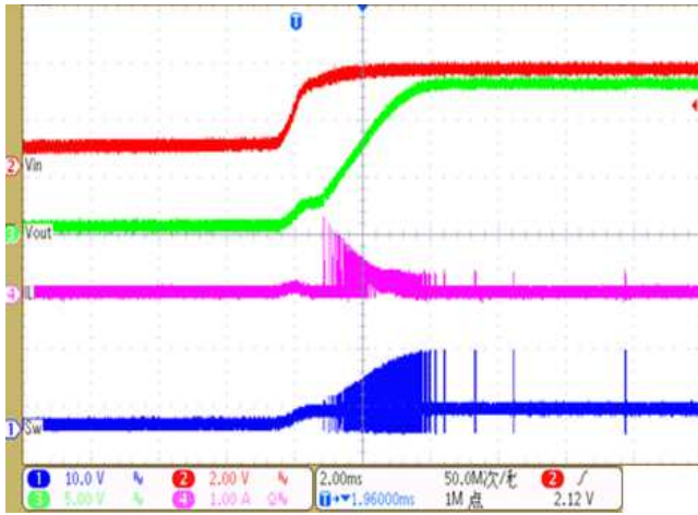
Figure 6. Power On @ No Load
