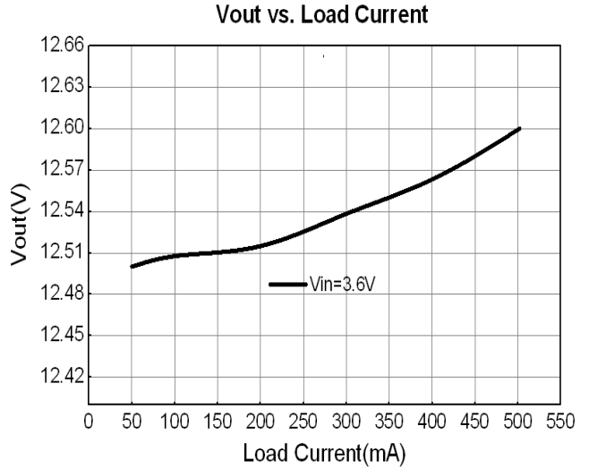
Figure 3. Load Regulation
