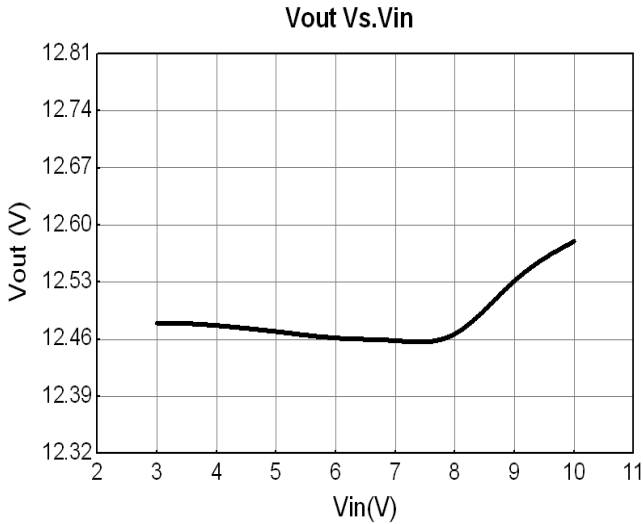
Figure 2. Line Regulation @ 200mA
