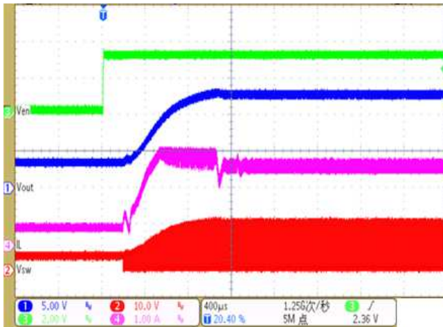
Figure 8. Enable Start Up @ Load=0.45A
