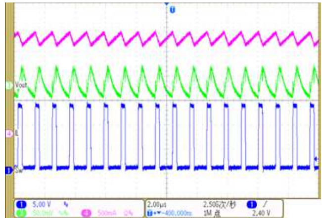
Figure 11. Ripple CCM mode @ Load=0.2A
