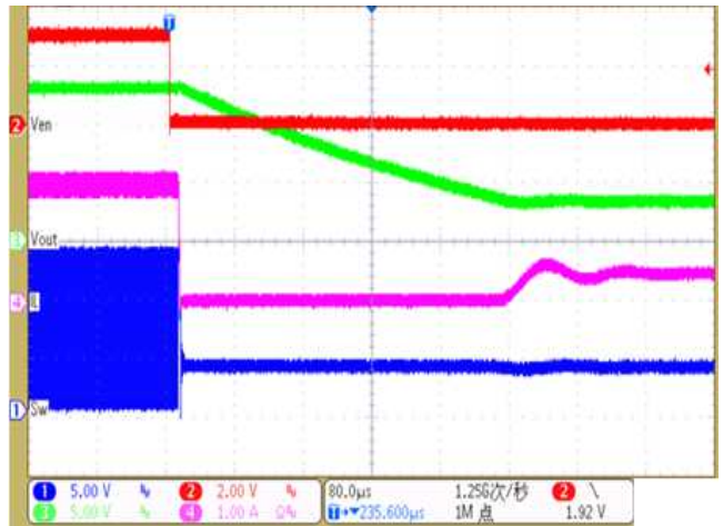
Figure 9. Enable Shut Down @ Load=0.45A
