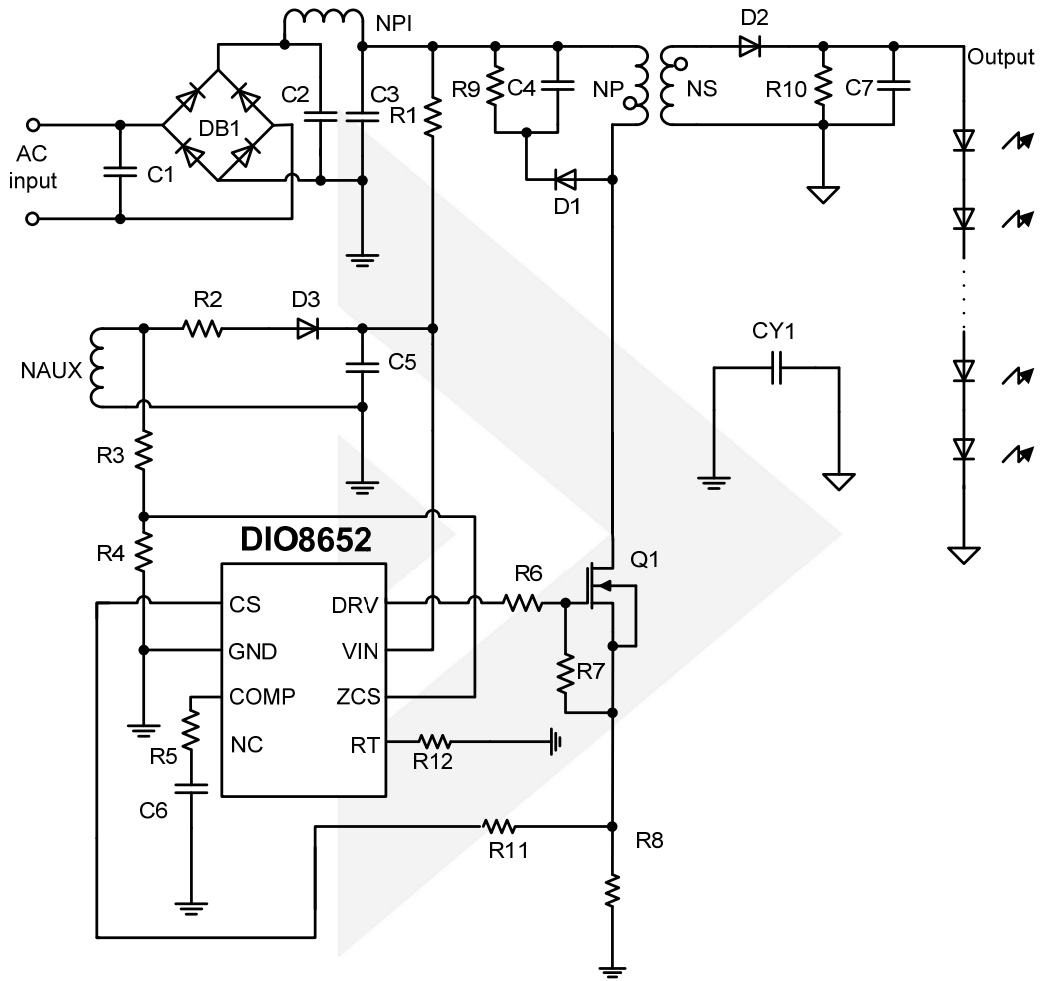
Figure 3 Typical Application
